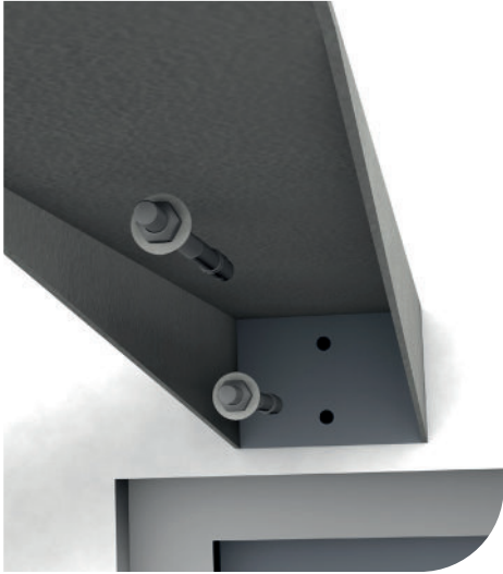
2. Install the first wall bracket.
