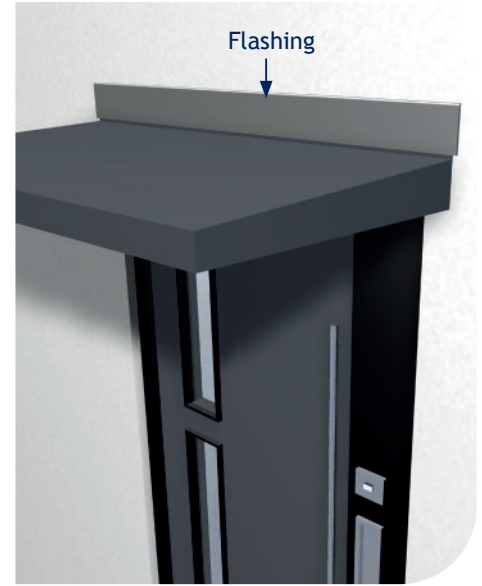
8. Finally, dress the top of canopy with lead or required flashing.
